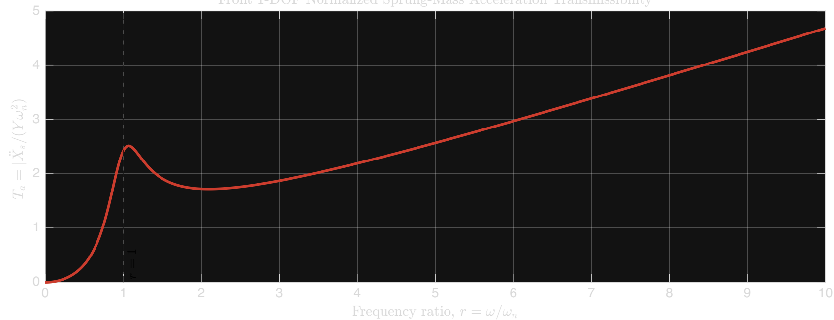
Front 1-DOF Normalized Sprung-Mass Acceleration Transmissibility
