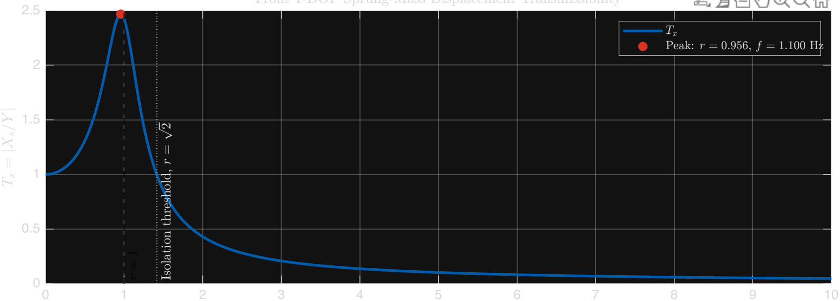
Front 1-DOF Normalized Sprung-Mass Acceleration Transmissibility
